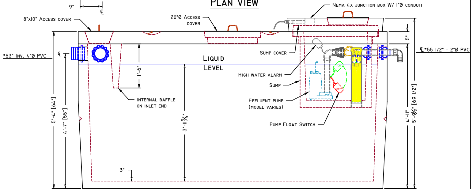
ELEVATION VIEW
