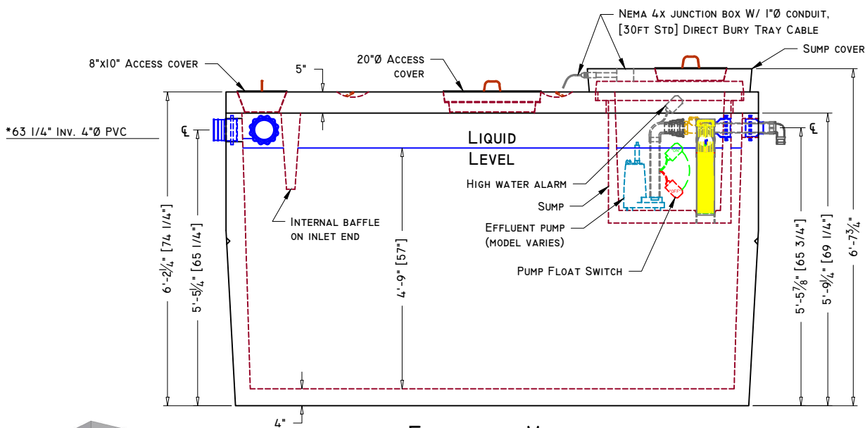
ELEVATION VIEW
